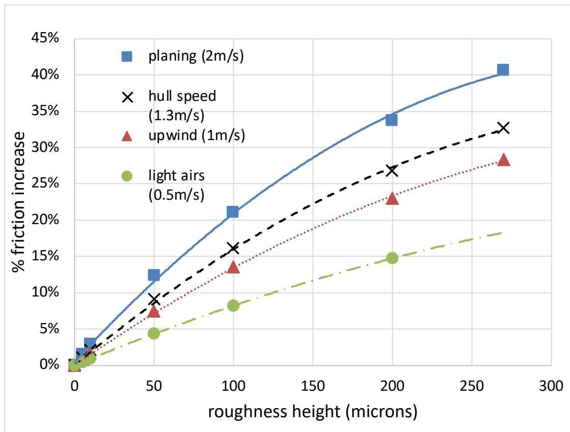
Figure 3: Effect of roughness height on friction (equation 10)
