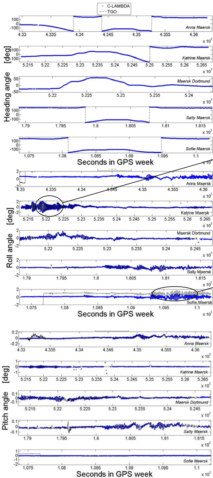
Figure 4 Time series of the attitude angles (Heading, Pitch, Roll) computed with the classical RTK approach using the TGO software (multi-epoch/dual-frequency) or applying the C-LAMBDA method (single-epoch/single-frequency) to the baselines formed by the onboard antennas.
